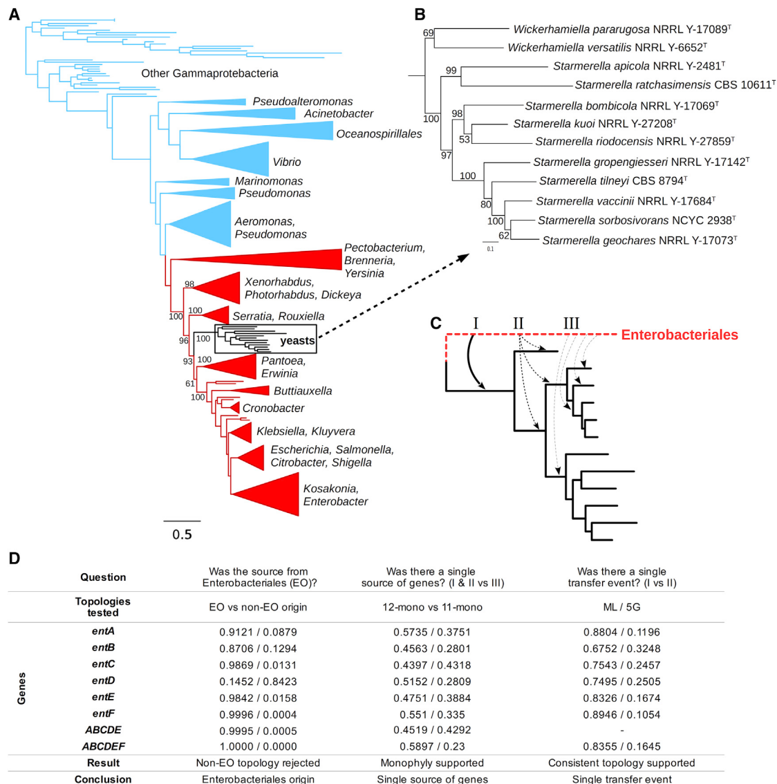
Figure 2. Yeast Siderophore Biosynthesis Originated from an Enterobacteriales Lineage
